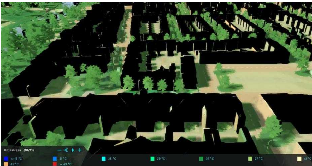
Figure 14 A close up image at 17:00, with the DPRA Heat Module, for the current situation in the Rivierenwijk (Tygron Geodesign Platform, 2020).
