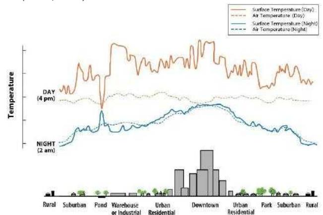
Figure 3 Urban Heat Island effect (EPA, 2019).
