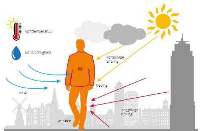
Figure 2 Schematic representation of the factors influencing the PET (HvA, 2020).
