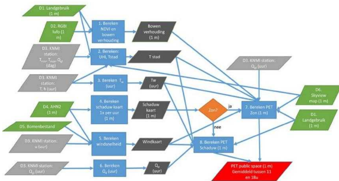
Figure 6 Flowchart of the data sources (D) and the calculations (blue) to measure the PET (RIVM, 2019).
